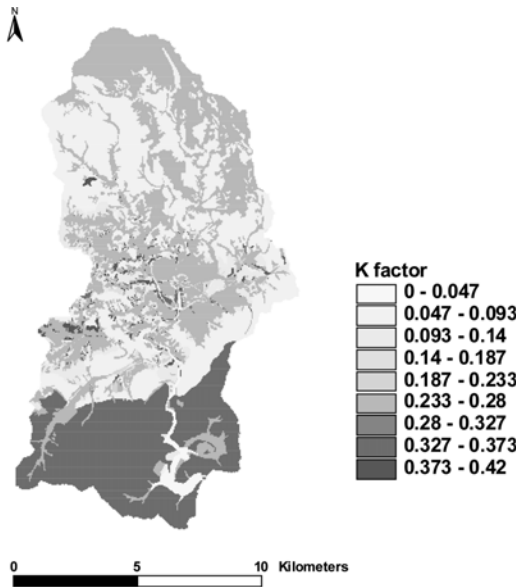
Fig. 5. K factor considering soil reconditioned agricultural fields at the Doam-dam watershed.
